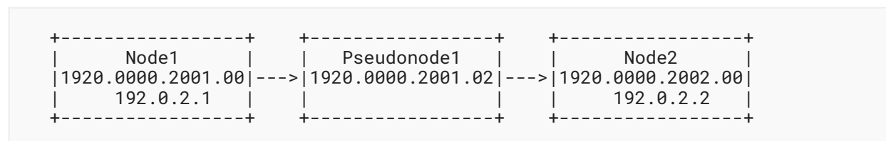
Figure 32: IS-IS Pseudonodes
