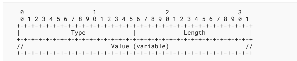
Figure 4: TLV Format
