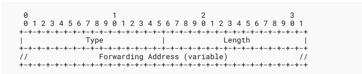
Figure 29: OSPF Forwarding Address TLV Format
