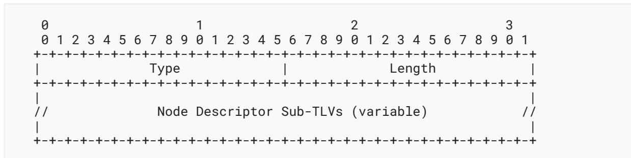
Figure 11: Remote Node Descriptors TLV Format
