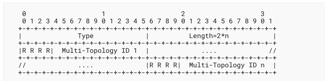
Figure 12: Multi-Topology Identifier TLV Format
